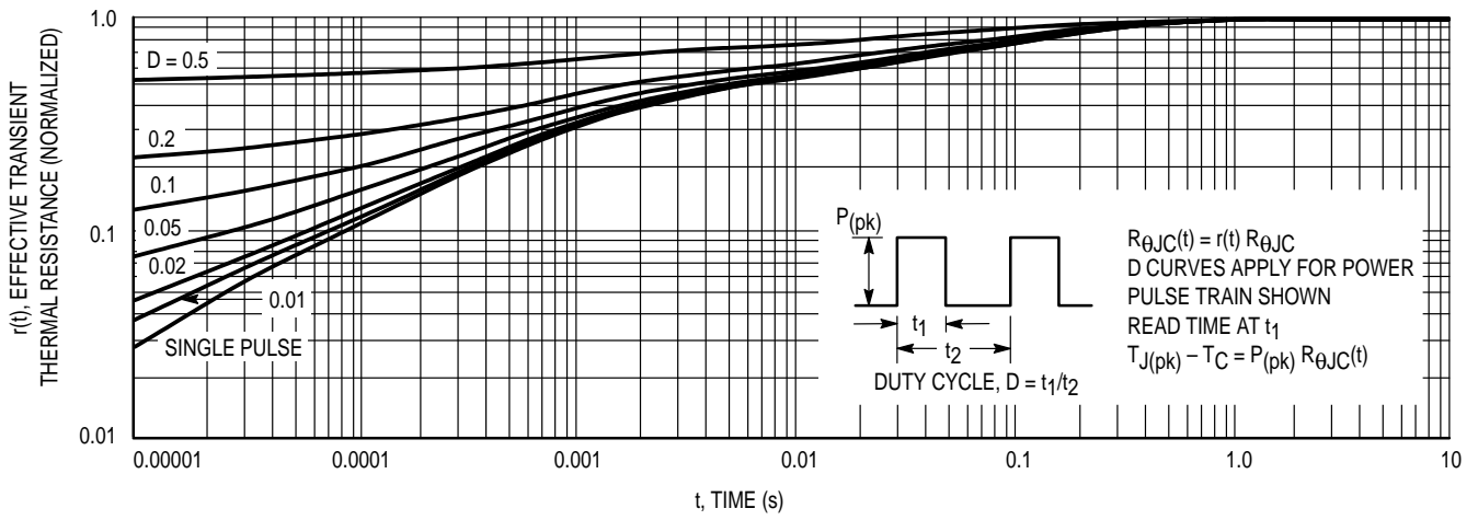
Figure 14. Thermal Response
